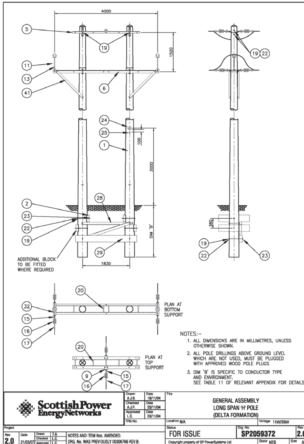
Figure 16 Delta Long Span “H” Pole Section or Section Angle (Drawing SP2059372)
